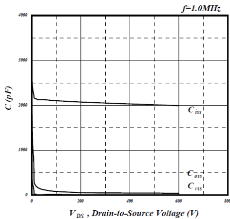
Figure 5. Capacitance Characteristics
